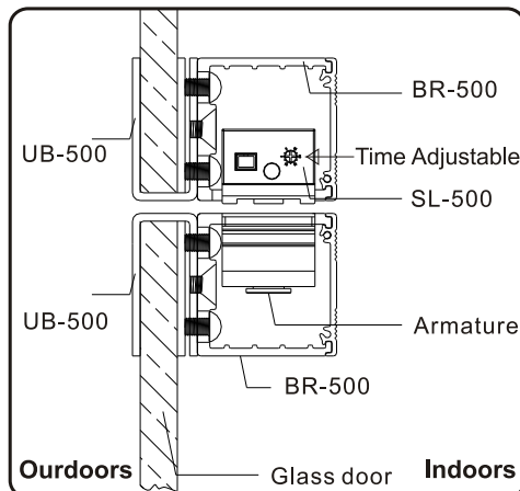
BR-500 bracket
