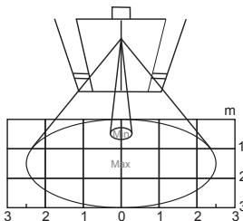
Inside out induction is invalid
