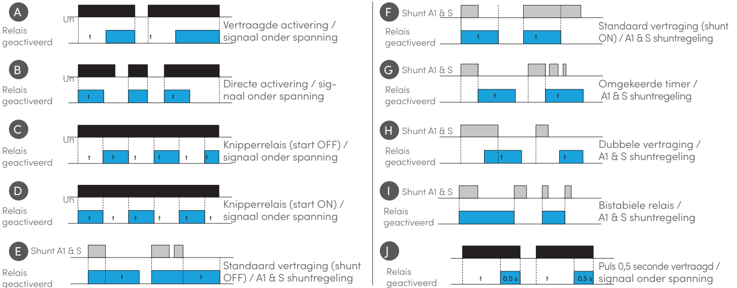
➤ LCTRD55U (multi-programma)
